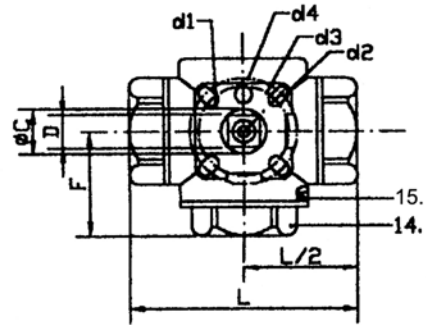
CLAMP ENDS
