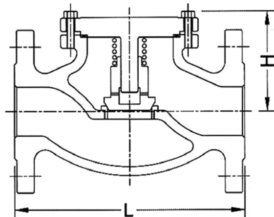
10K/20K 2-1/2" ~ 10"
