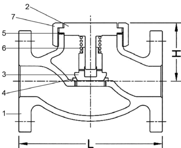
16K/20K 1/2" ~ 2"
