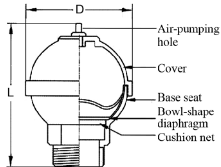
▲ Thread end (AIT) Without Pressure Gauge
