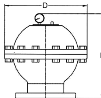
▲ Flange end (AIF) With Pressure Gauge
